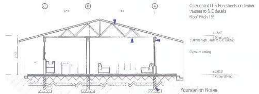
X-X Building Section 1:100
