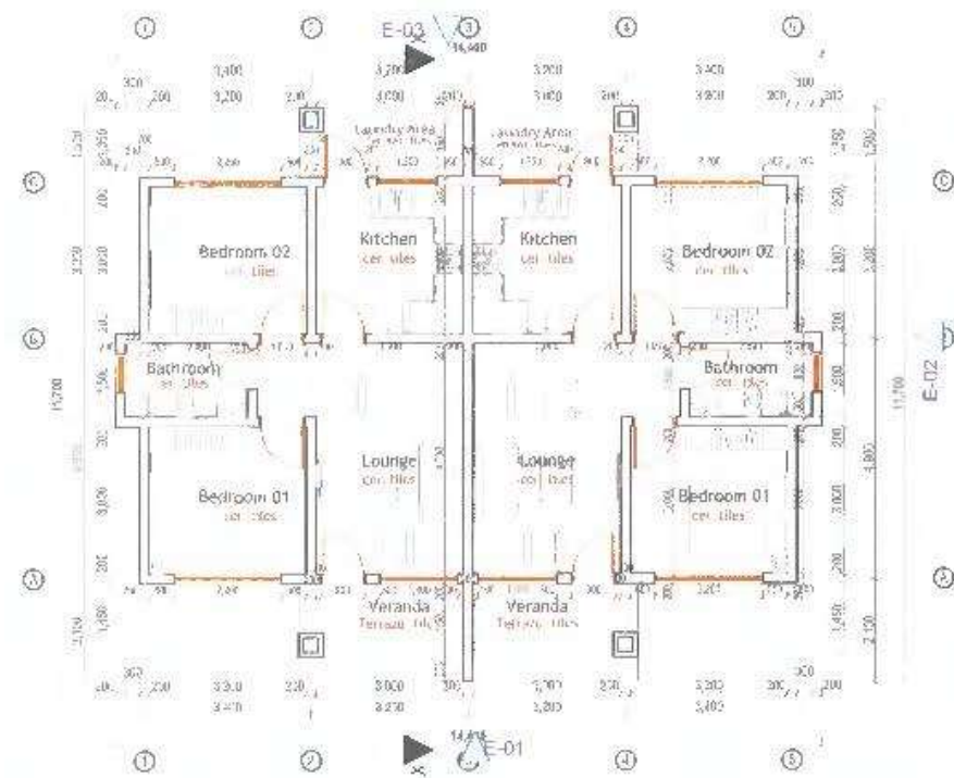
0 Ground Floor 1:100
